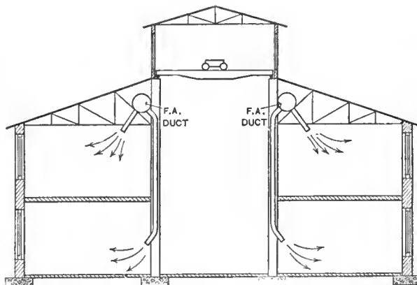
FIG. 1. AN ARRANGEMENT OF DUCTS SUITABLE FOR MONITOR ROOF CONSTRUCTION
